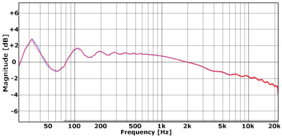
Gap 4 \mu m, Modern tape at 7.5 ips, IEC15, input -12dB
