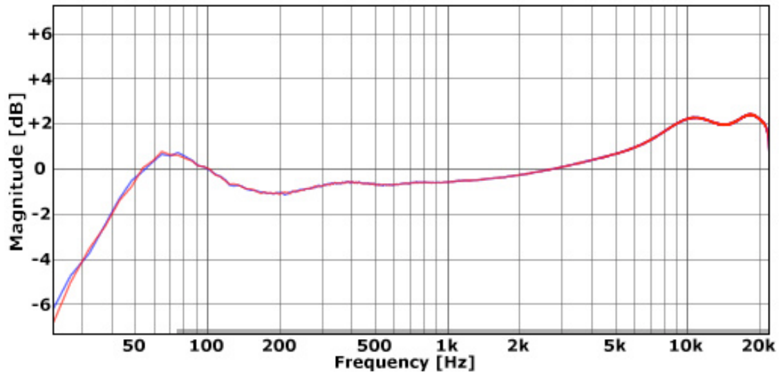
Gap 2 \mu m, Modern tape at 15 ips, IEC15, input -12dB
