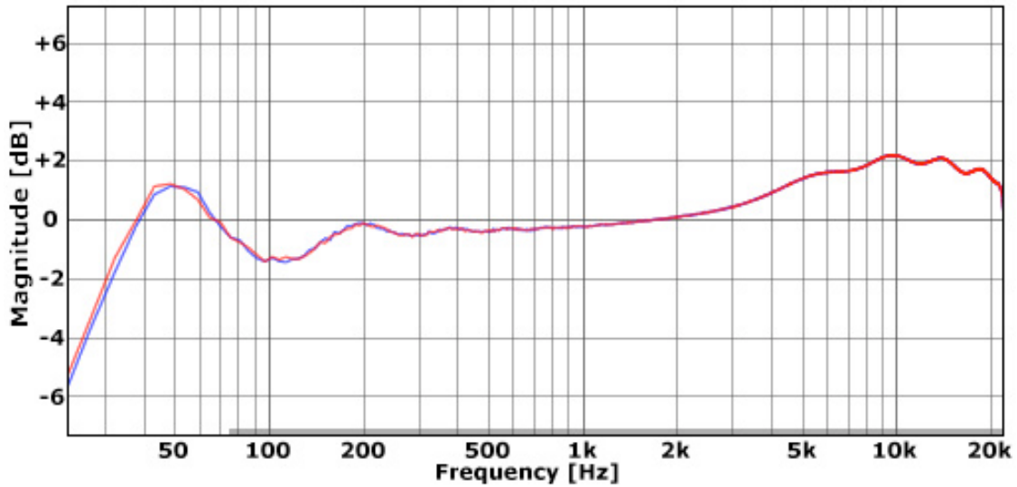
Gap 3 \mu m, Modern tape at 7.5 ips, IEC15, input -12dB
